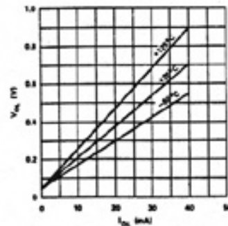
OUTPUT CURRENT VS. OUTPUT VOLTAGE OUTPUT LOW
