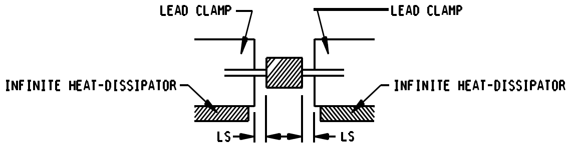
FIGURE 6. Mounting conditions.
