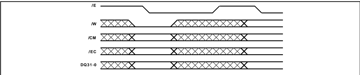
Figure 3: Write Cycle
