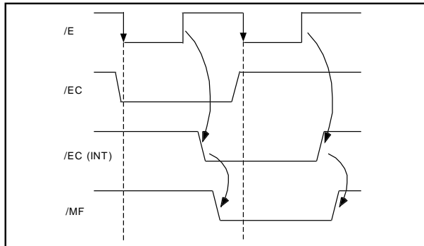
Figure 5: /EC(Int) Timing Diagram
