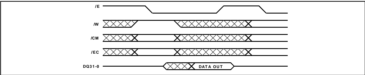
Figure 2: Read Cycle
