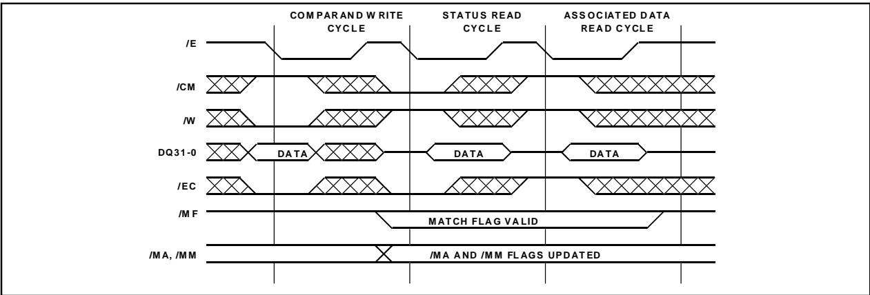
Figure 4: Cycle to Cycle Timing Example
