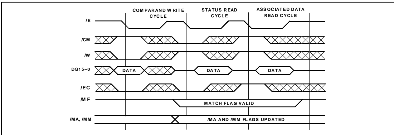
Figure 5: Cycle to Cycle Timing Example
