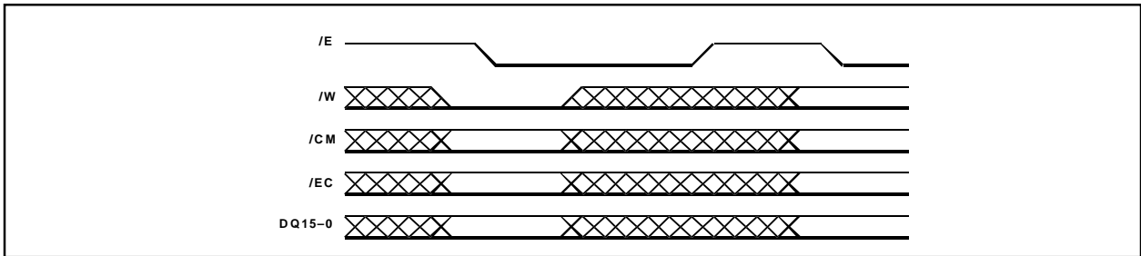
Figure 4: Write Cycle
