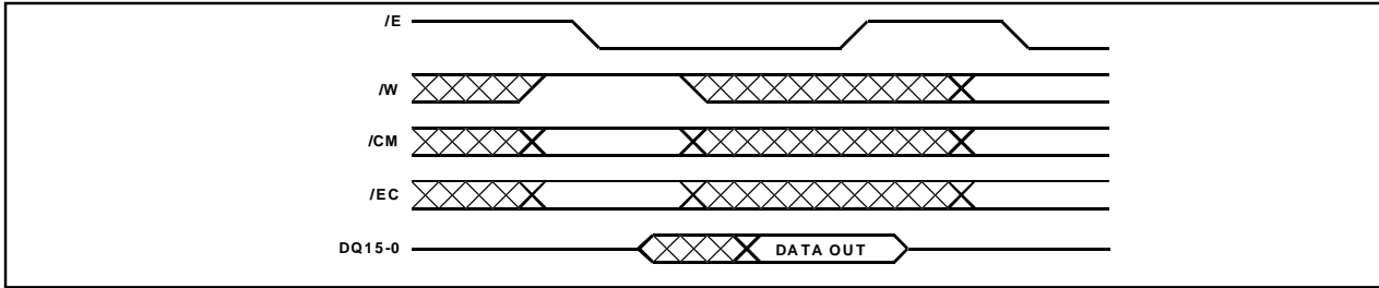
Figure 3: Read Cycle
