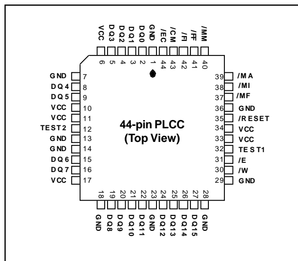
PINOUT DIAGRAM
