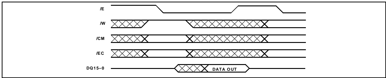
Figure 3: Read Cycle
