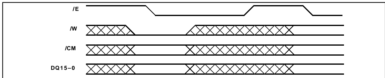
Figure 4: Write Cycle
