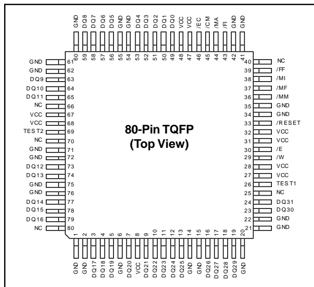
Pinout Diagram
