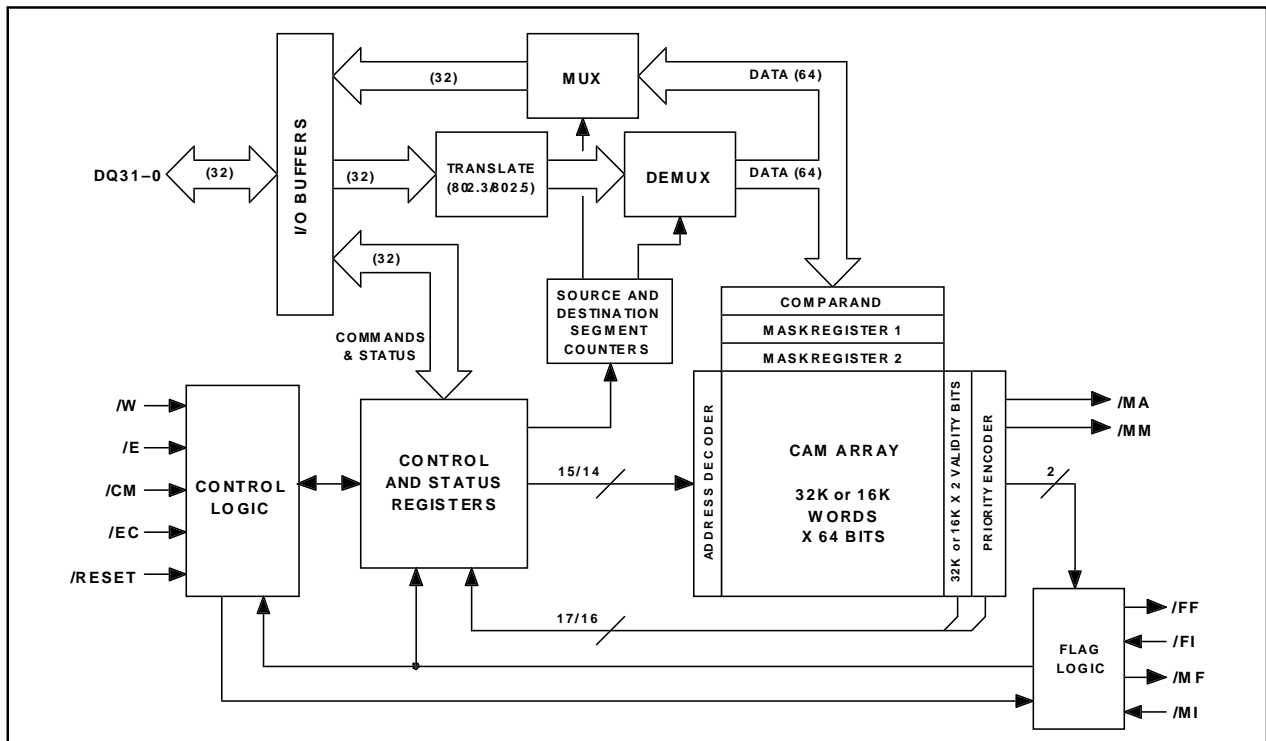
Block Diagram
