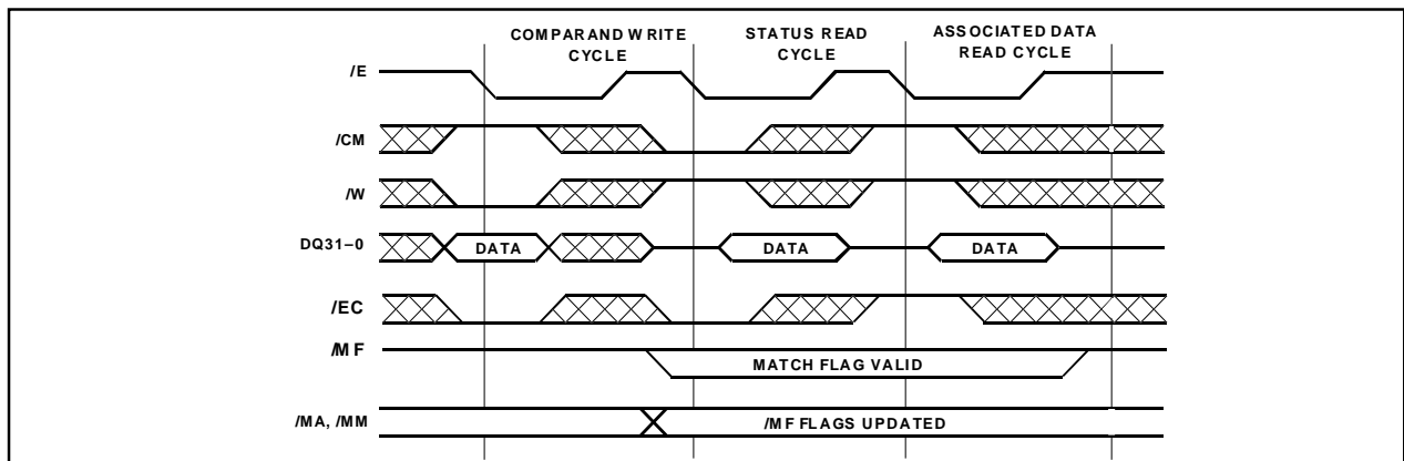
Figure 5: Cycle to Cycle Timing Example
