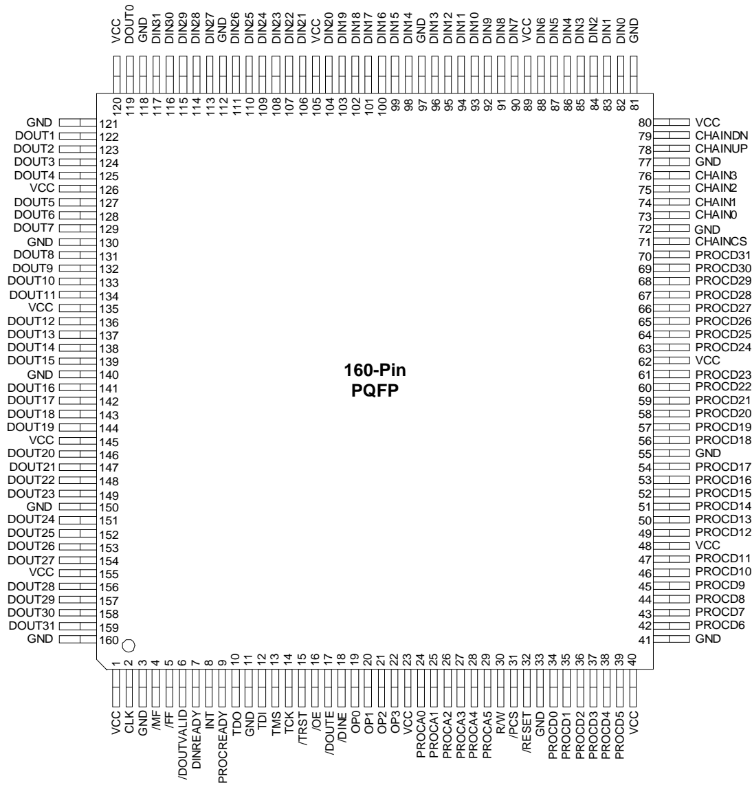
Figure 2: 160-Pin PQFP (Top View)
