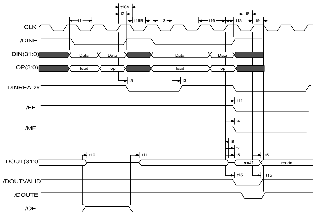
Figure 5: Sync Port Cycle
