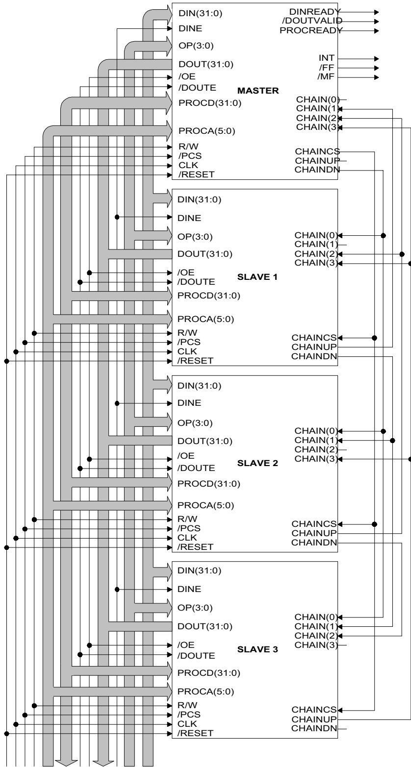
Figure 3: Device Chaining
