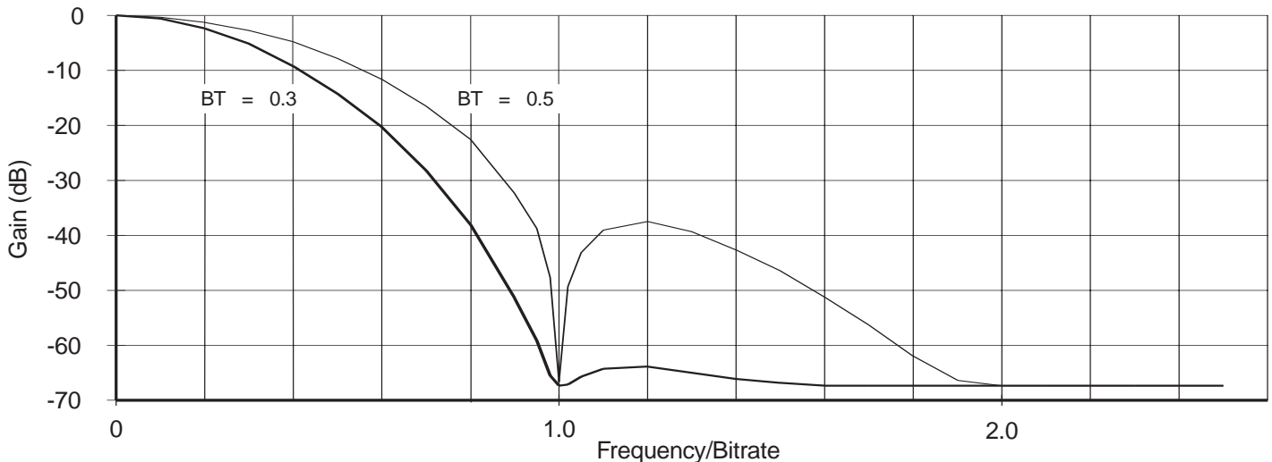
Figure 11: Tx Output Spectrum (Random Data)
