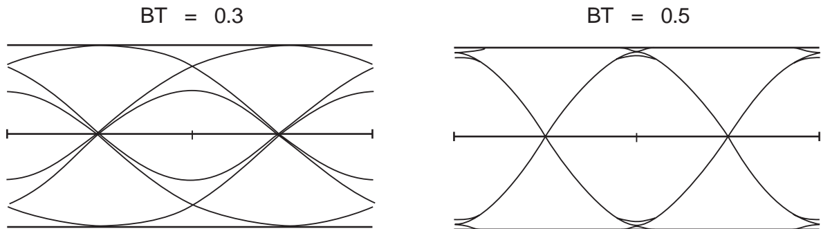
Figure 10: Typical Transmit Eye Patterns
