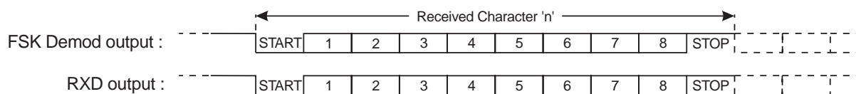
Figure 8: FSK Operation without Rx Data Re-timing (CLK always high)
