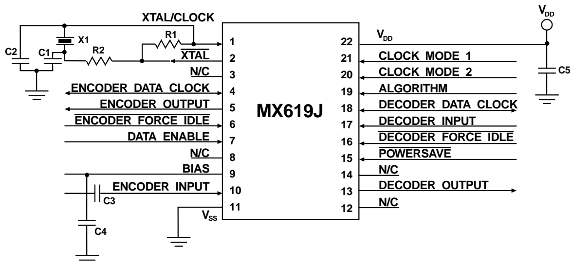
Figure 2: Recommended External Components for Typical Application
