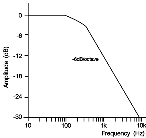
Figure 11: Principal Integrator Response
