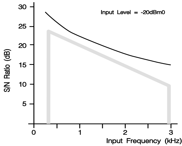
Figure 10: S/N vs. Input Frequency (32kbps)
