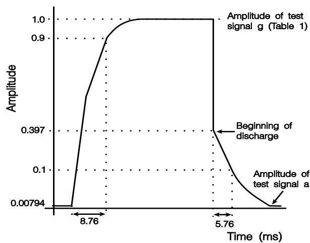
Figure 12: Compand Envelope
