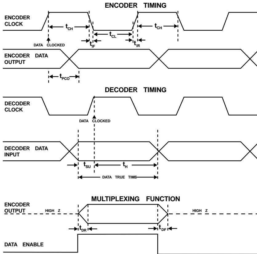
Figure 14: CODEC Timing
