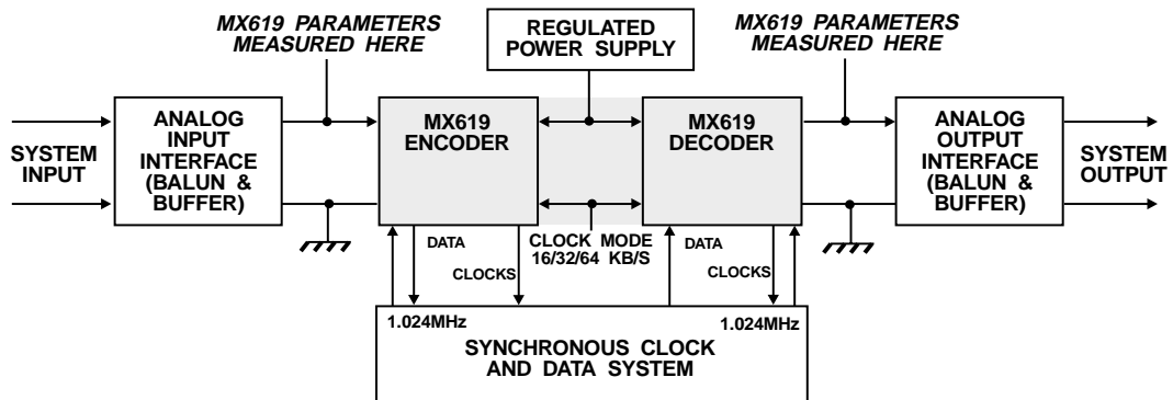
Figure 3: System Configuration using the MX619
