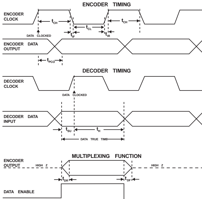
Figure 14: CODEC Timing
