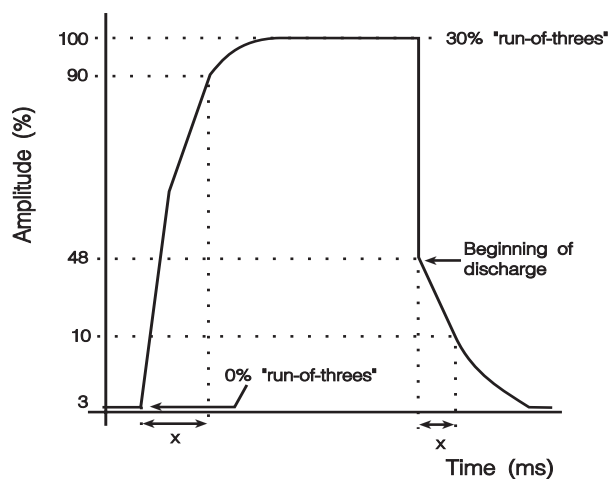
Figure 12: Compand Envelope
