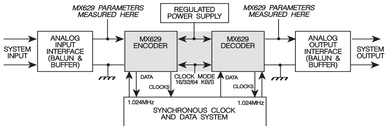
Figure 3: System Configuration using the MX629
