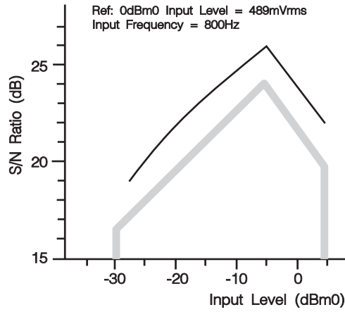
Figure 7: S/N vs. Input Level (32kbps)
