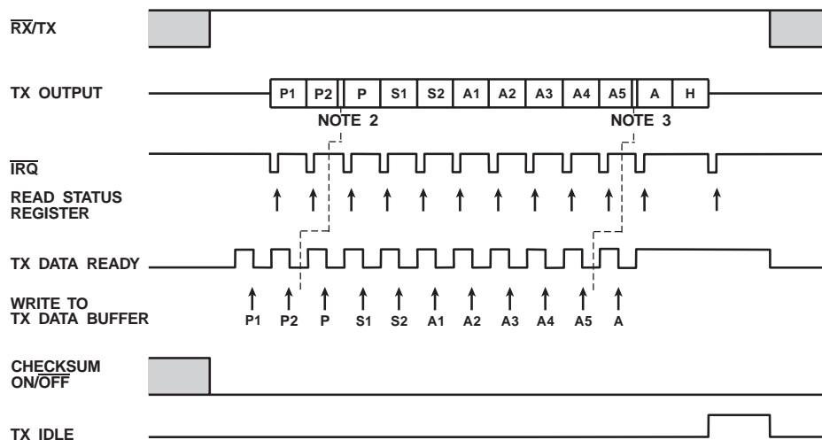
Figure 8: TX One Message, TX Checksum Not Enabled
