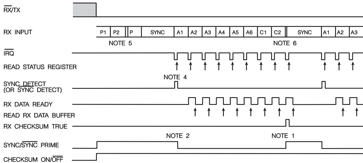
Figure 4: Modem Timing
