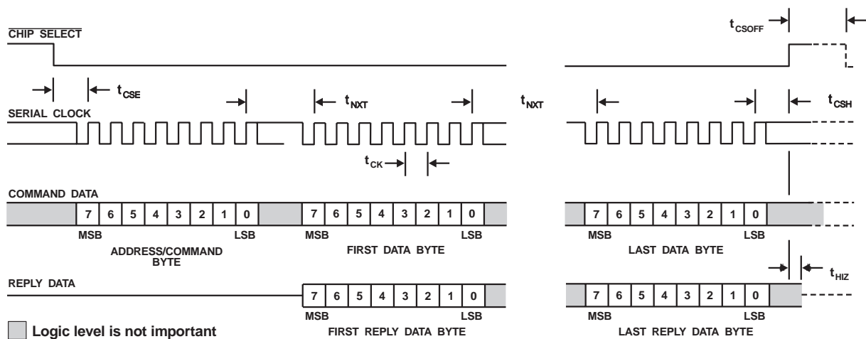
Figure 11: C-BUS Timing Information
