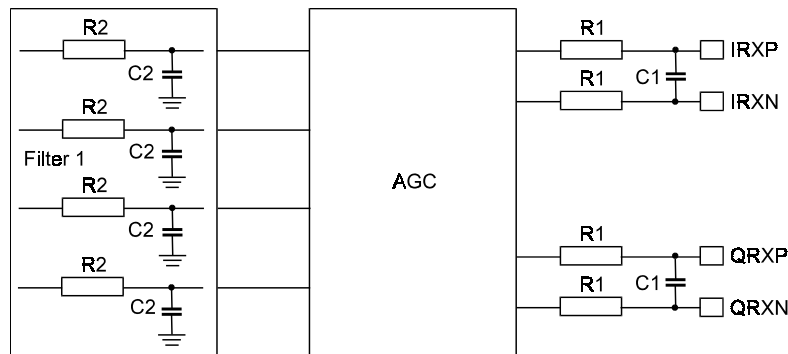
Figure 2: Recommended External Components - Rx Input
