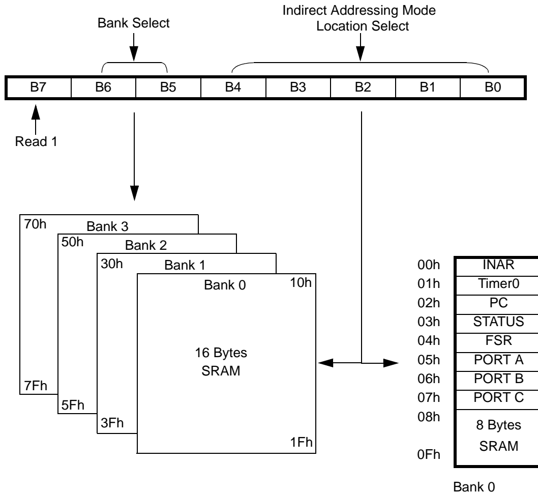
FIGURE 2. Data Memory Configuraion
