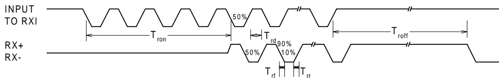
Figure 1. Reception Timing
