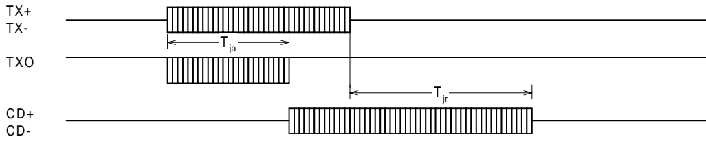
Figure 5. Jabber Timing
