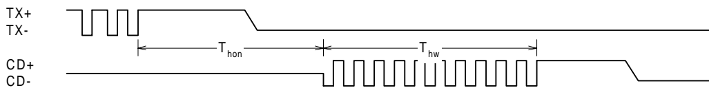
Figure 3. Heartbeat Timing
