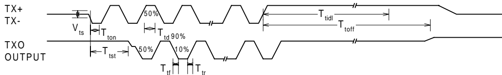
Figure 2. Transmission Timing
