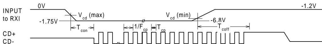
Figure 4. Collision Timing
