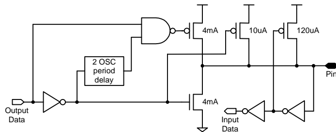
8051 Standard Pin
