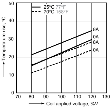
3.-(2) Coil temperature rise (1 Form A 1 Form B) Tested sample: DE1a1b-5V Quantity: n=6 Ambient temperature: 25°C to 70°C 77°F to 158°F
