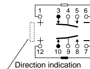
2 coil latching (Reset condition)
