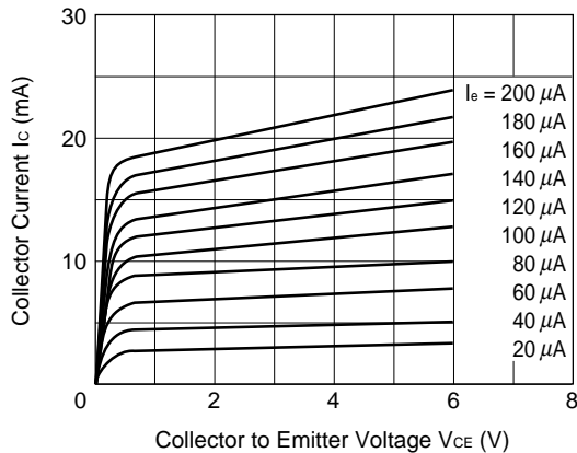
I C - V CE CHARACTERISTICS
