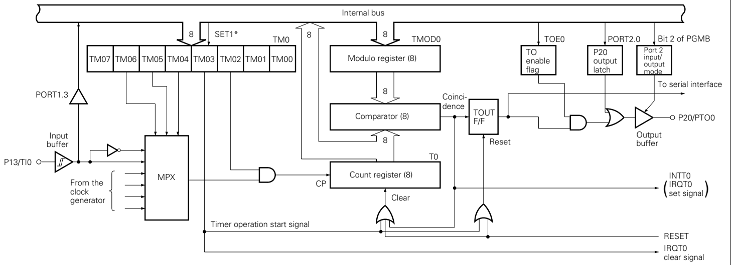
Fig. 6-5 Timer/Event Counter Block Diagram
