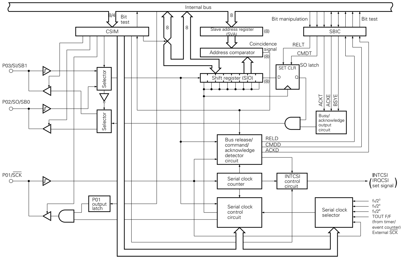
Fig. 6-6 Serial Interface Block Diagram
