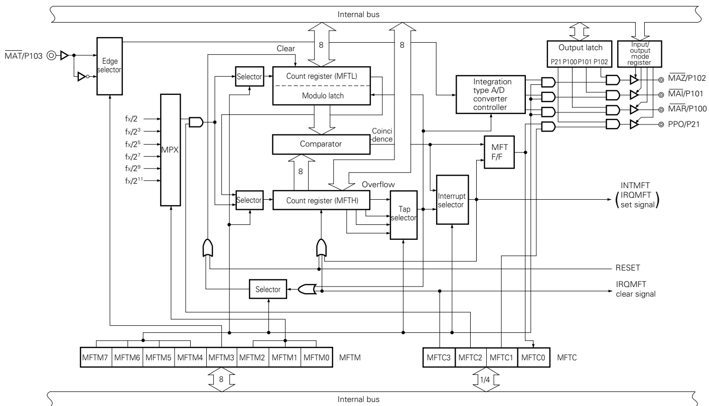
Fig. 6-8 Multi-Function Timer Block Diagram
