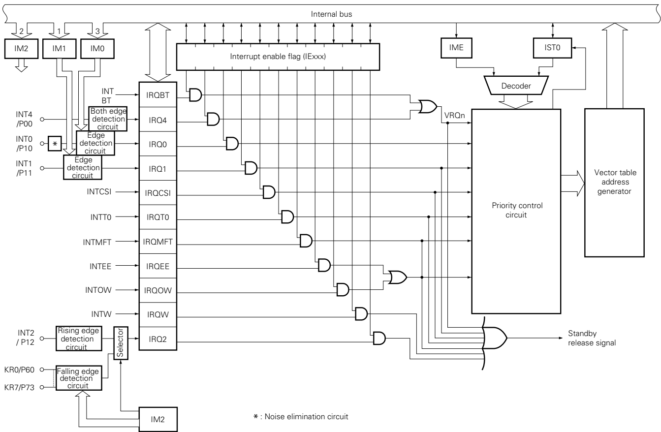
Fig. 7-1 Interrupt Control Circuit Block Diagram
