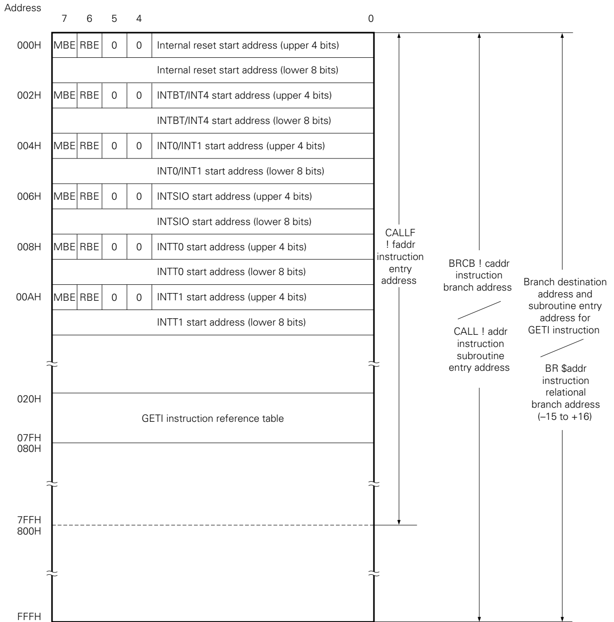
Fig. 4-1 Program Memory Map (3/3)
