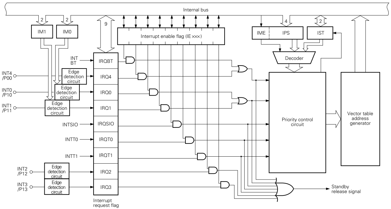
Fig. 6-1 Interrupt Control Block Diagram
