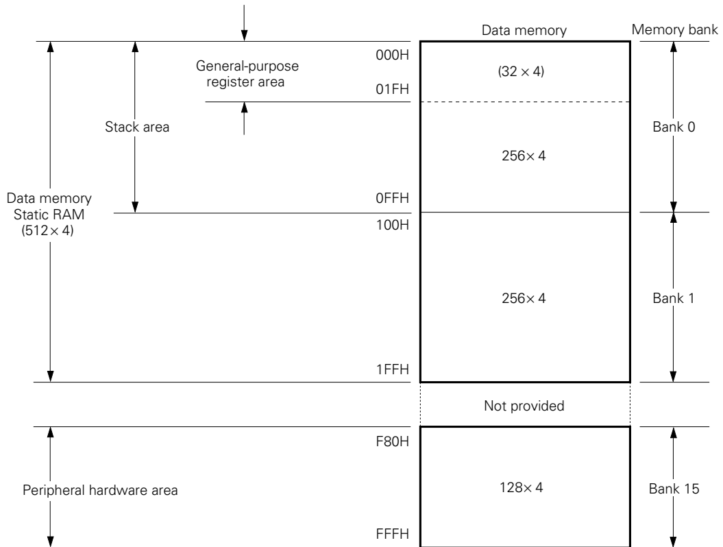
(a) μPD75108A
