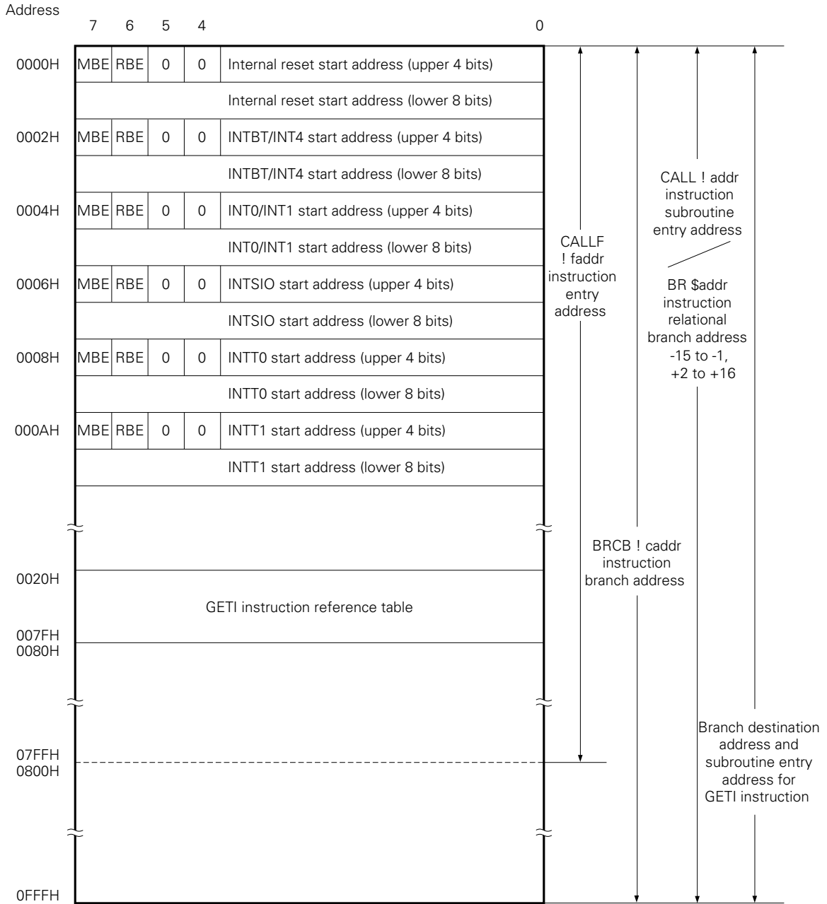
Fig. 4-1 Program Memory Map (2/2)
