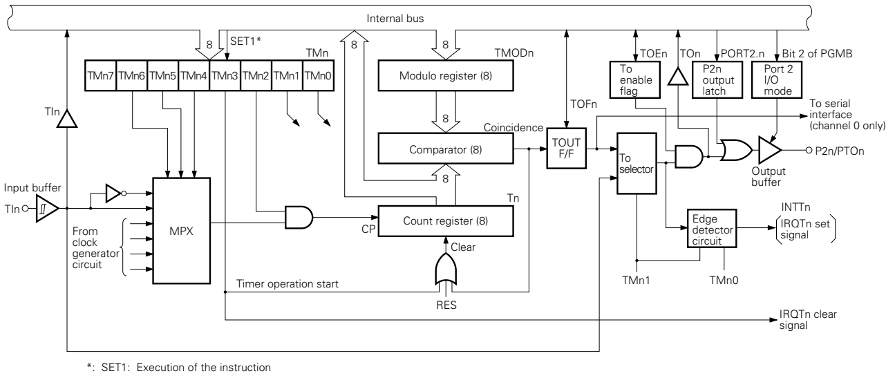
Fig. 5-4 Timer/Event Counter Block Diagram (n = 0, 1)
