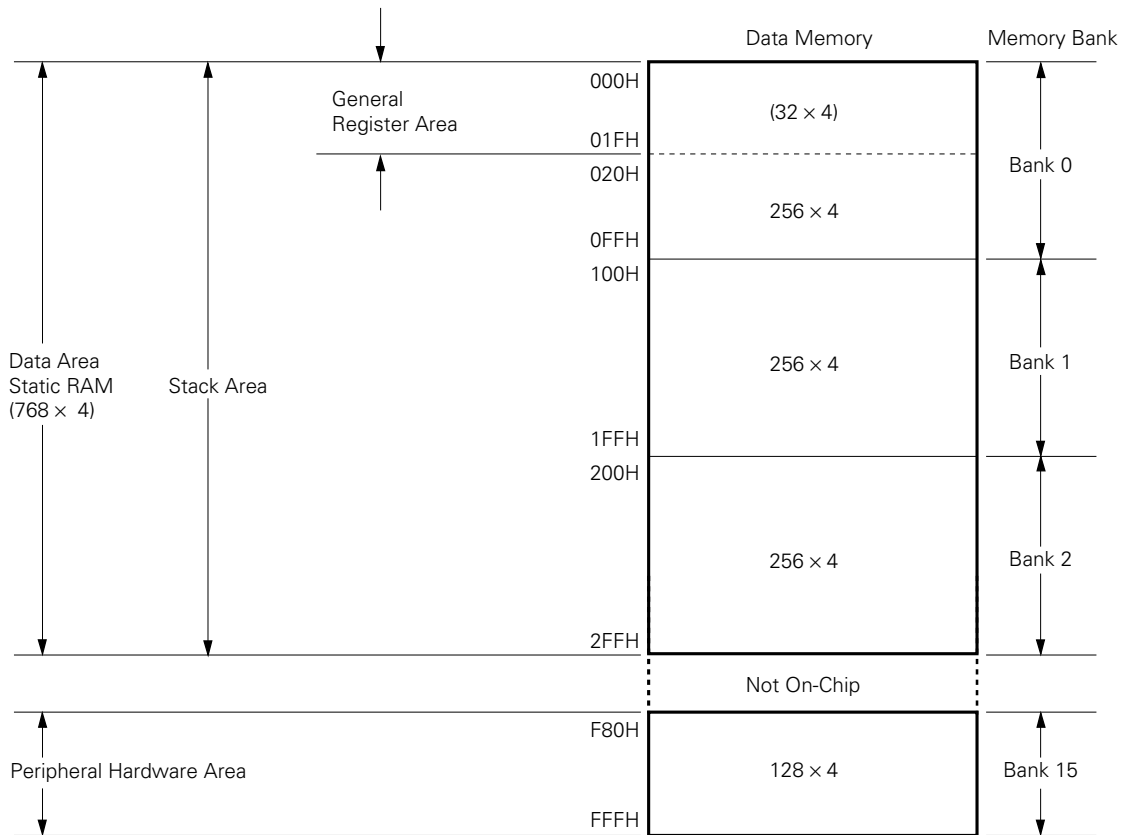
Fig. 4-2 Data Memory Map (1/2) (a) \mu PD75117H
