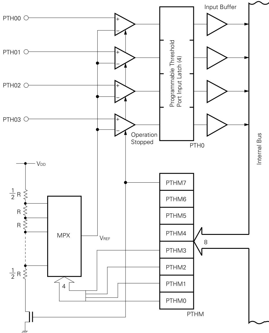
Fig. 5-6 Programmable Threshold Port Block Diagram
