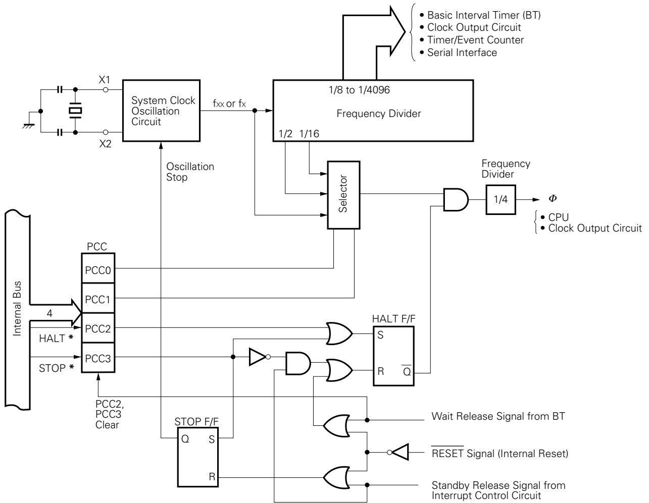
Fig. 5-1 Clock Generator Block Diagram
