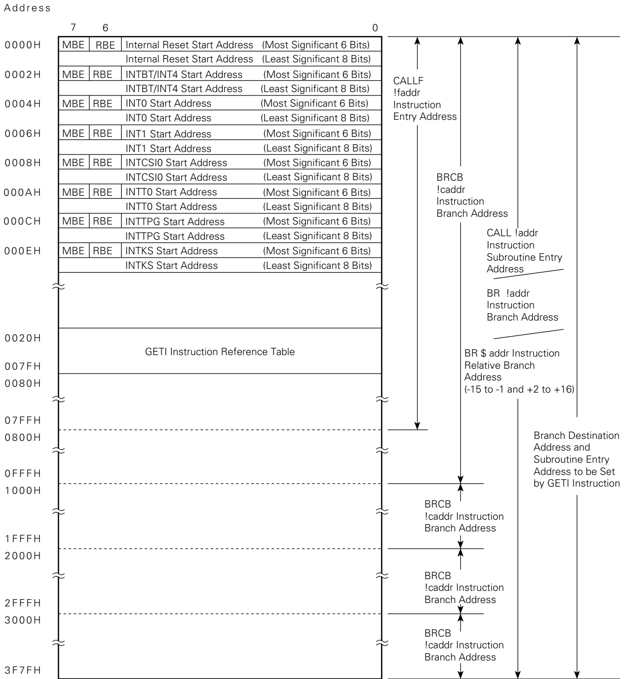
Fig. 4-1 Program Memory Map
