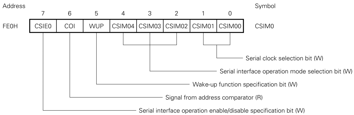
Fig. 4-40 Format of Serial Operation Mode Register 0 (CSIM0) (1/3)
