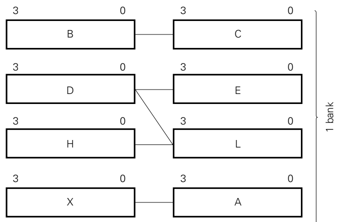
Fig. 3-6 Register Pair Format
