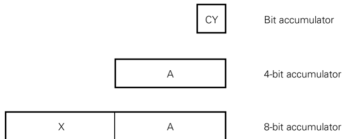
Fig. 3-7 Accumulators
