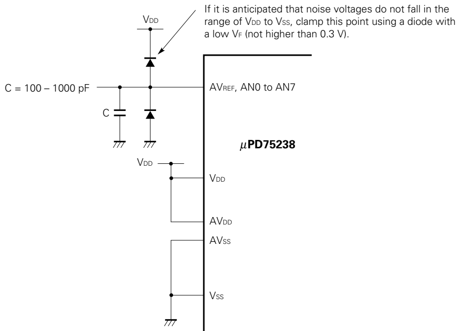
Fig. 4-66 Analog Input Pin Connection
