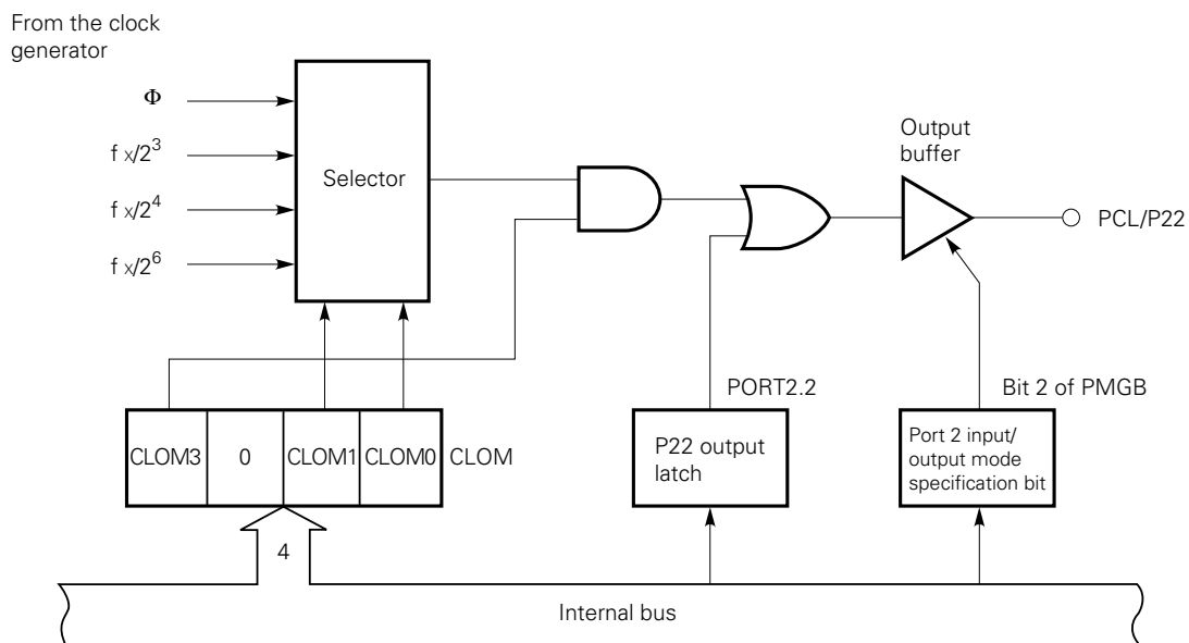
Fig. 4-20 Configuration of the Clock Output Circuit
