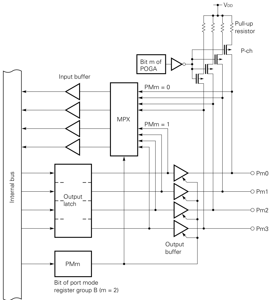
Fig. 4-4 Configuration of Port 2
