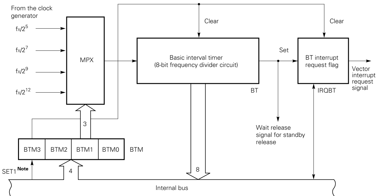
Fig. 4-23 Configuration of the Basic Interval Timer
