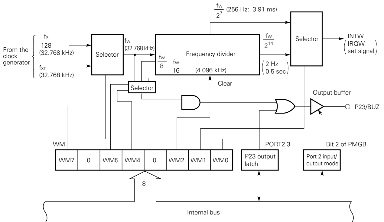
Fig. 4-29 Block Diagram of the Clock Timer
