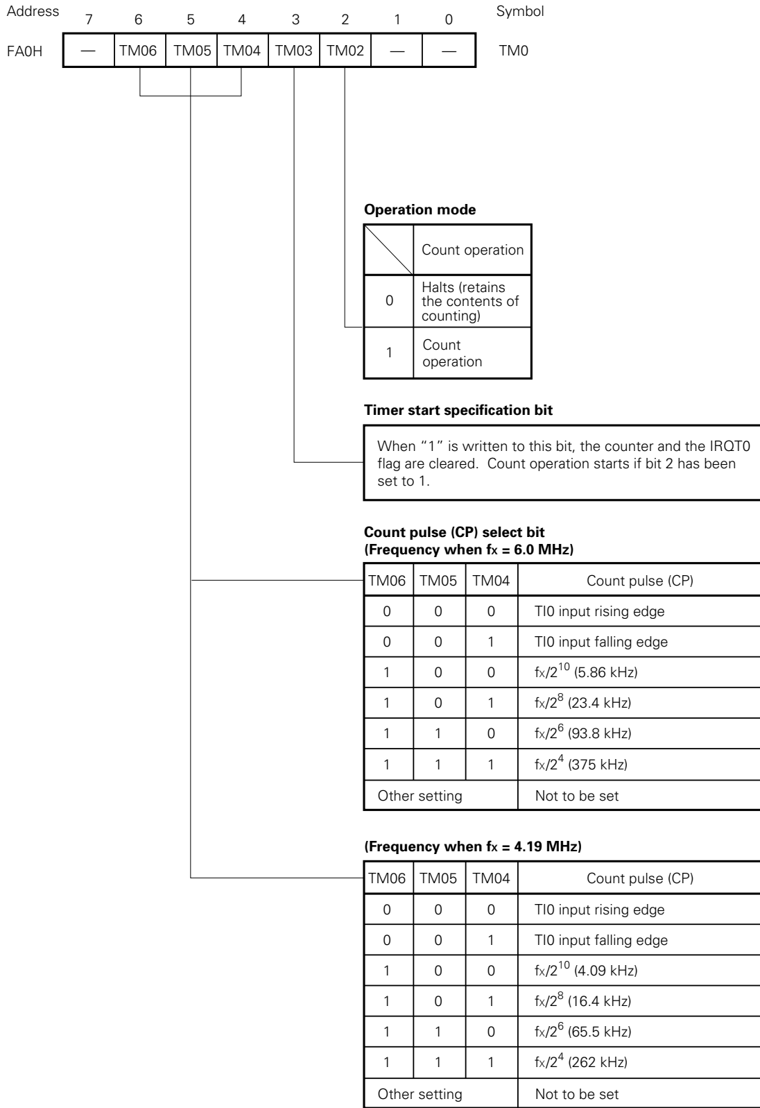
Fig. 4-27 Format of the Timer/Event Counter Mode Register
