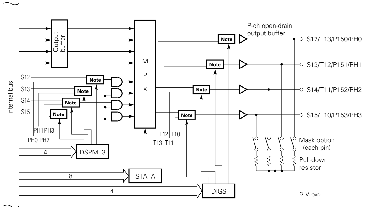
Fig. 4-11 Configuration of Ports 15 and H
