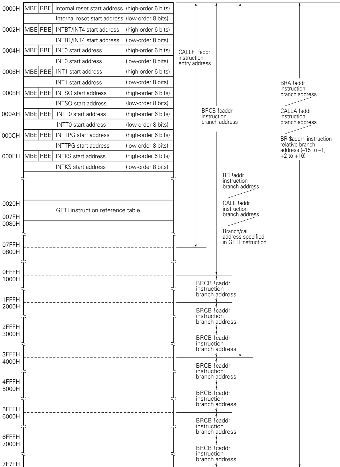
Fig. 3-2 Program Memory Map
