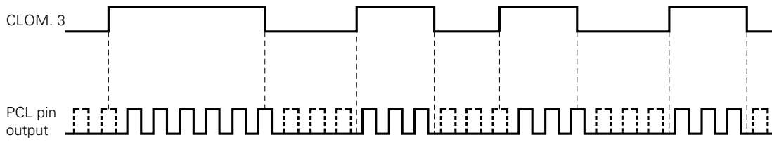
Fig. 4-22 Application to Remote Control Output
