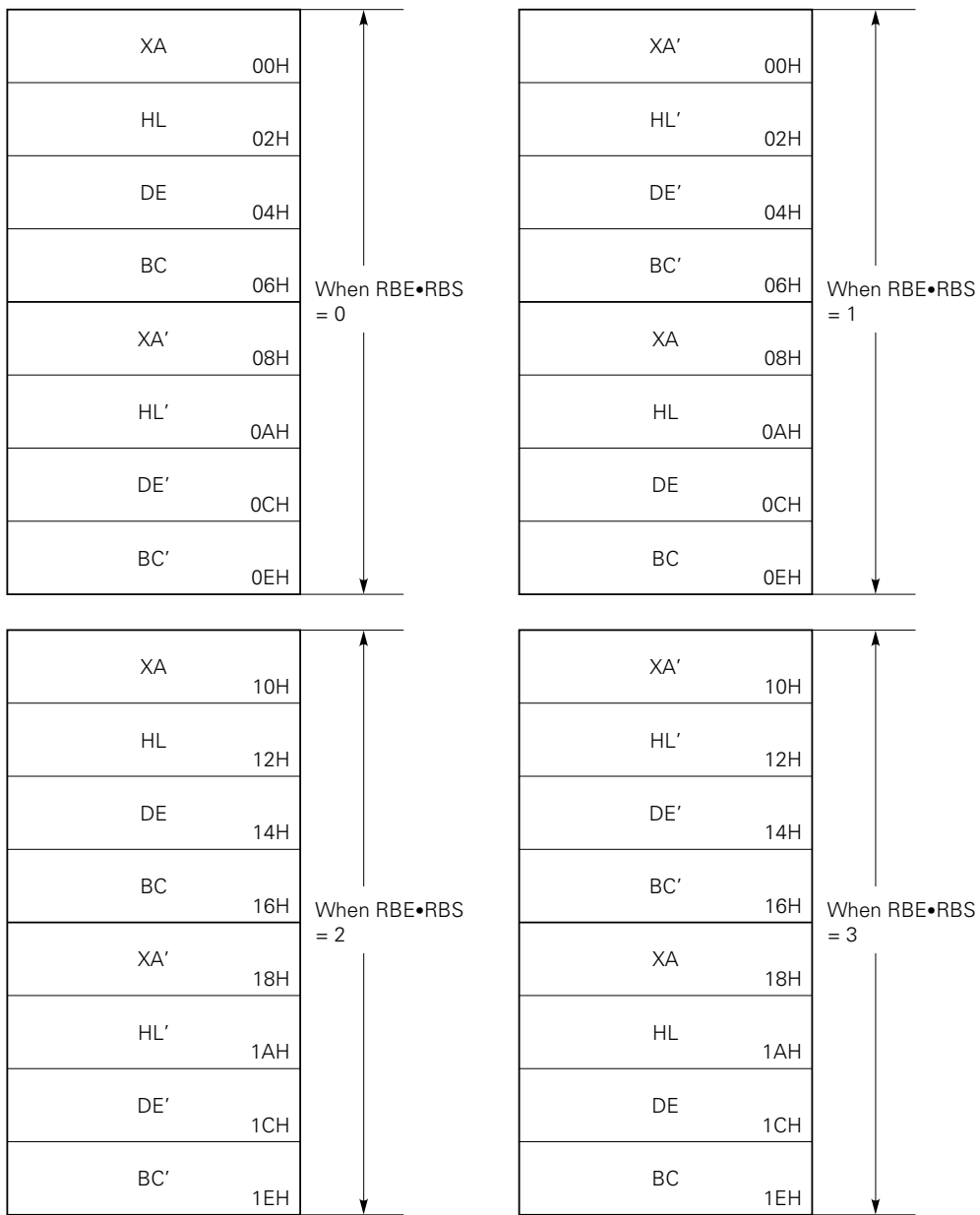
Fig. 2-3 General Register Configuration (8-Bit Processing)
