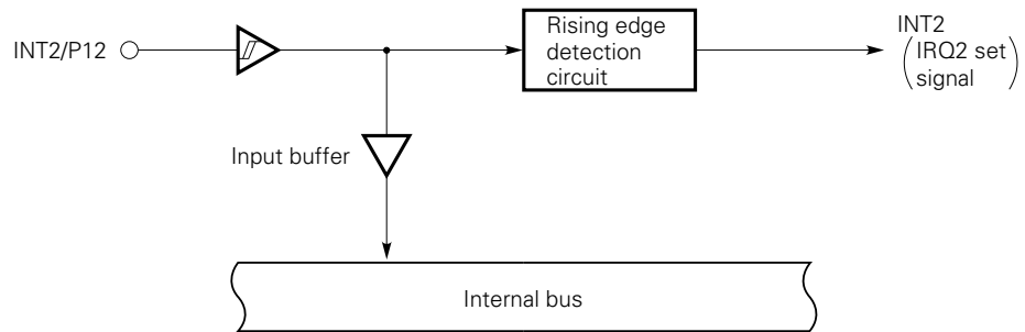
Fig. 5-3 Configuration of INT2
