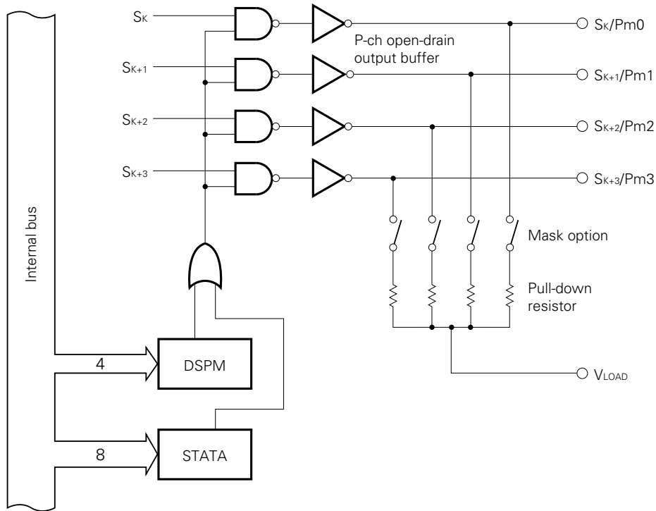
Fig. 4-9 Configuration of Ports 12 and 13
