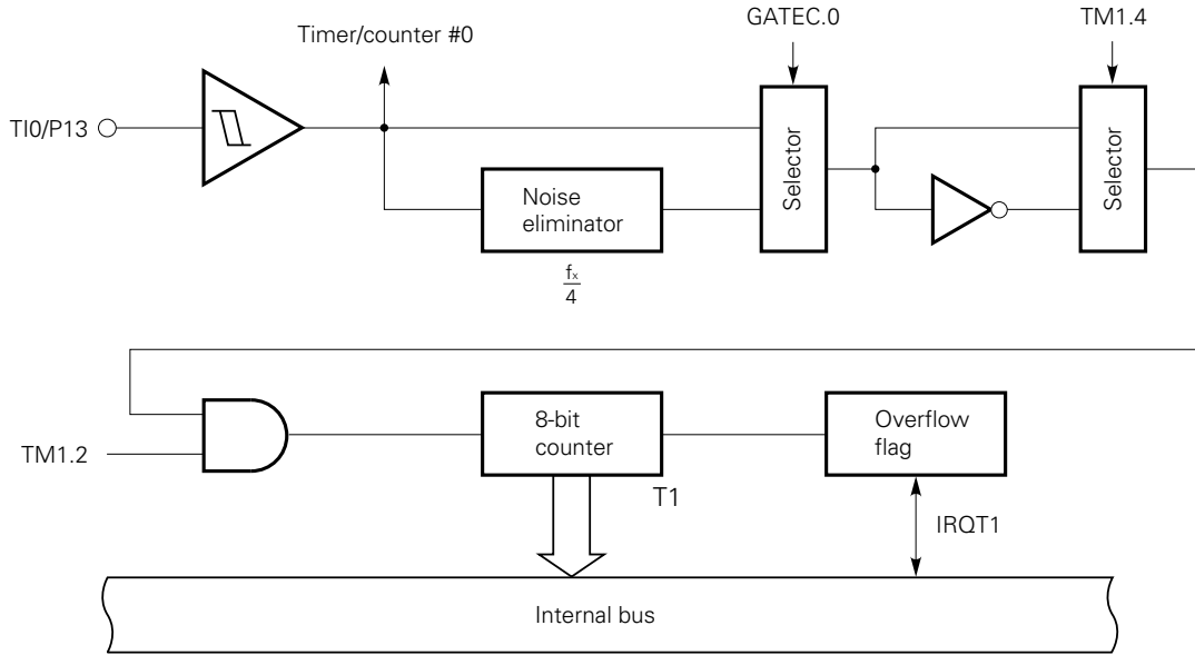
Fig. 4-36 Block Diagram of the Event Counter
