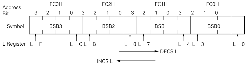
Fig. 5-8 Bit Sequential Buffer Format
