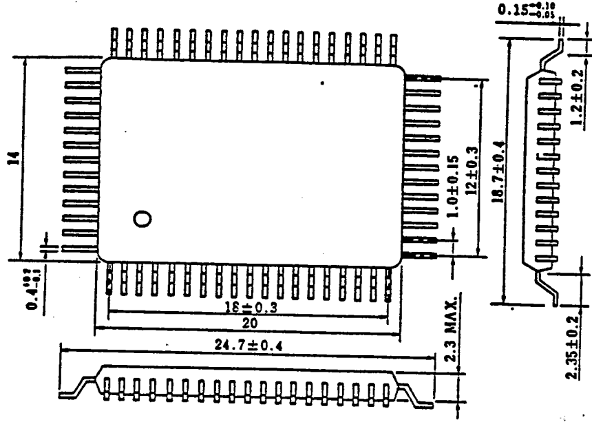
bent leads (12)
