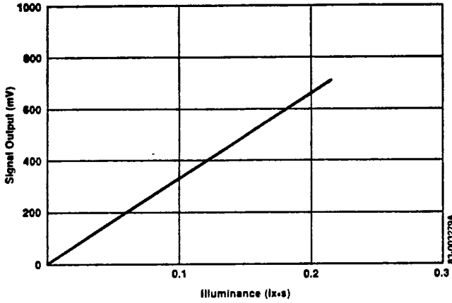
Signal Output
