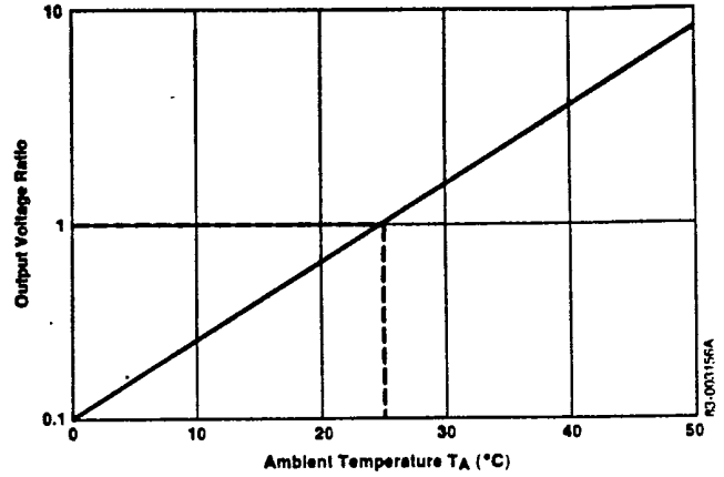
Dark Signal
