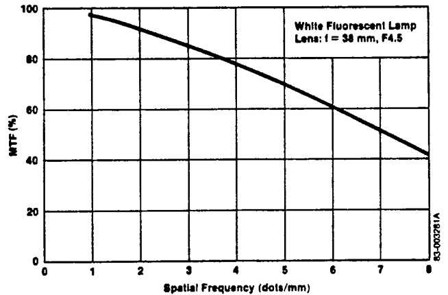
MTF
