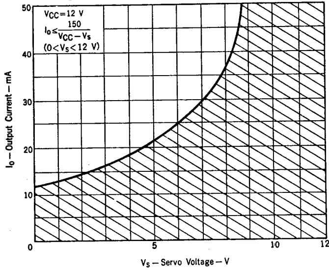
Fig. 2 OUTPUT CURRENT vs. SERVO VOLTAGE
