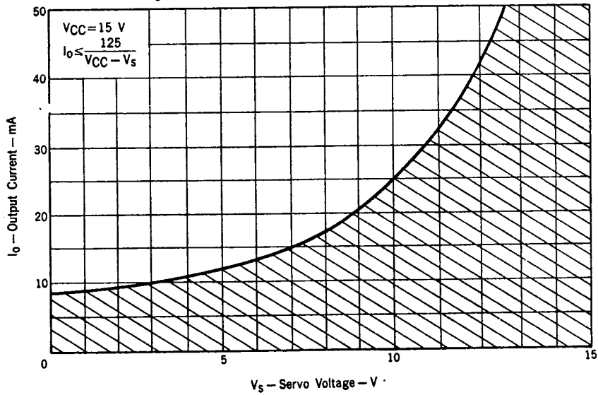
Fig. 3 OUTPUT CURRENT vs. SERVO VOLTAGE
