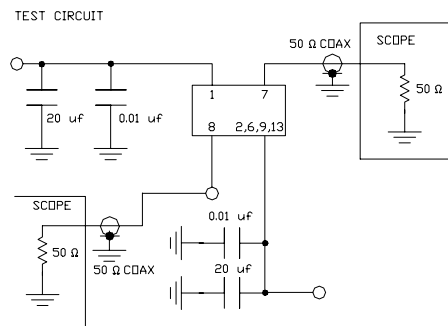
TEST CIRCUIT USES A SPLIT SUPPLY OF +2V AND -3V FOR EASE OF TESTING.
