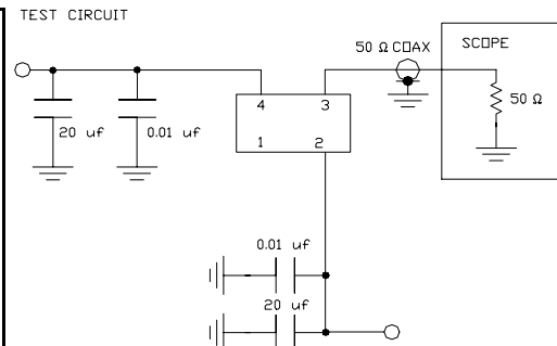
TEST CIRCUIT USES A SPLIT SUPPLY OF +2V AND -2.5V FOR EASE OF TESTING.
