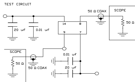
TEST CIRCUIT USES A SPLIT SUPPLY OF +2V AND -3V FOR EASE OF TESTING.
