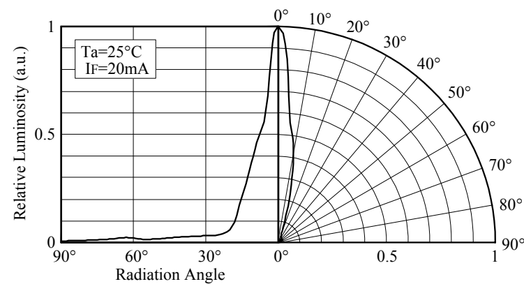
■ Directivity (NSPB300A)
