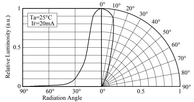
■ Directivity (NSPB510(S))
