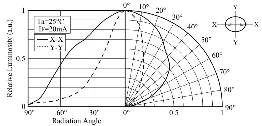
■ Directivity (NSPB546BS)
