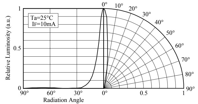
■ Directivity (NSPE590S)
