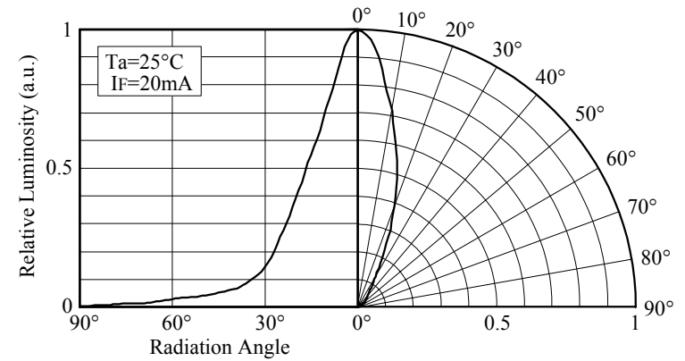
■ Directivity (NSPG310A)
