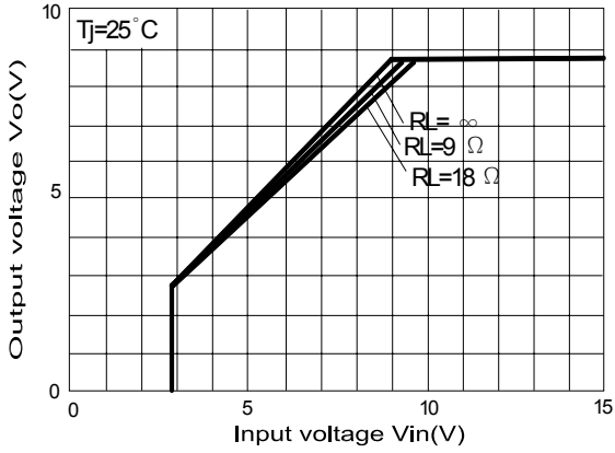
Output Voltage vs. Input Voltage(L1481T-9)
