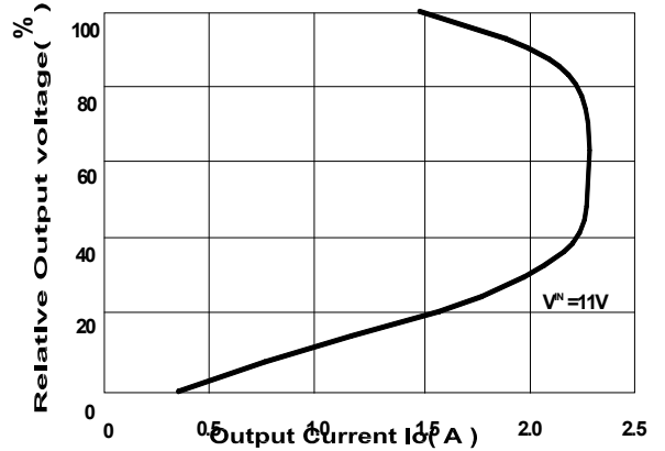
Overcurrent Protection Characteristics (Typical Value)(L1481T-9)
