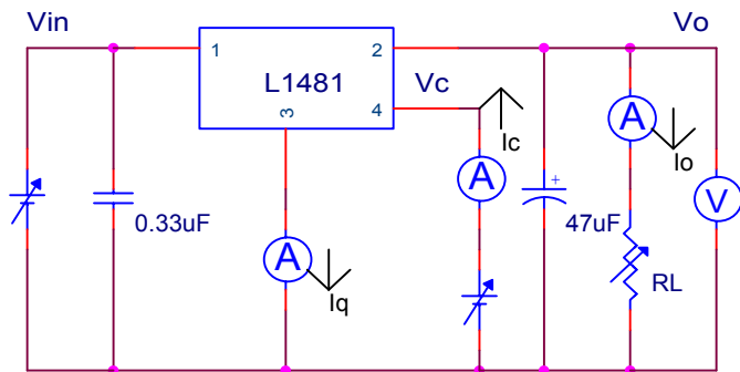
Fig.1 Test Circuit
