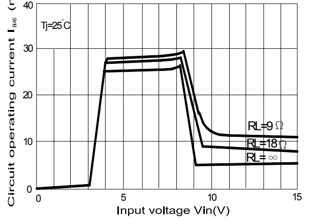
Circuit Operating current vs. Input Voltage (L1481T-9)
