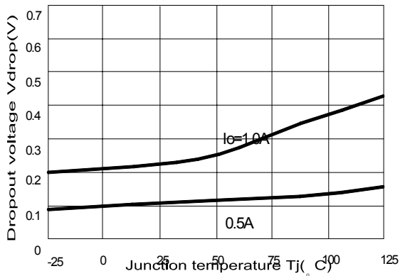
Dropout Voltage vs. Junction Temperature(Tj) (L1481T-9)
