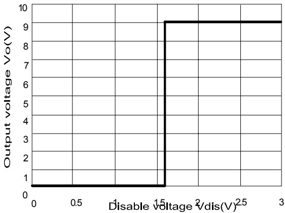
Output Voltage vs. Disable Voltage(L1481T-9)
