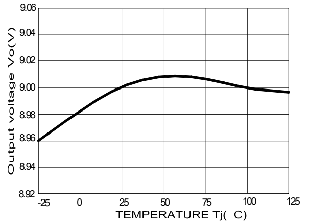
Output Voltage vs. Temperature(Tj)(L1481T-9)
