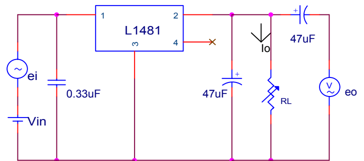
Fig.2 Test Circuit of Ripple Rejection
