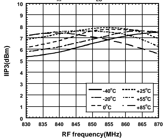
IIP3 vs. RF frequency
