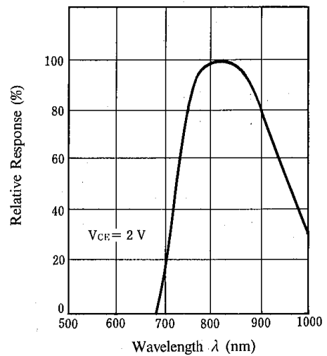
Spectral Response (T a =25°C)
