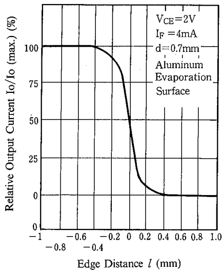
Output Current vs. Edge Distance ( T_a = 25^\circ\text{C} )
