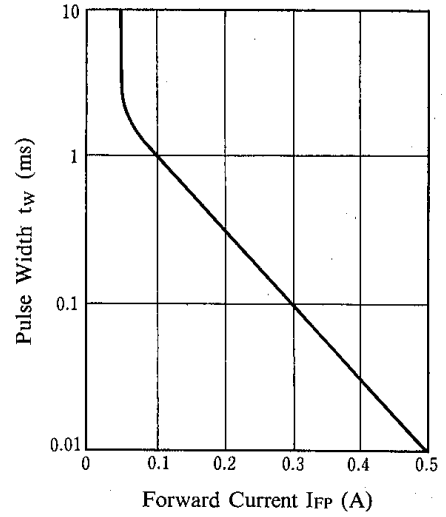
Pulse Width vs. Forward Current
