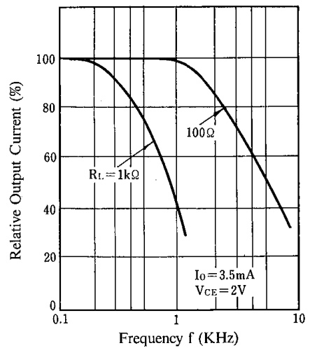
Output Current vs. Frequency (T a =25°C)
