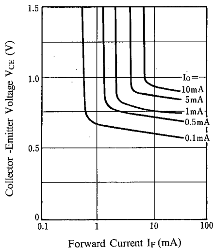
V CE Saturation (T a =25°C)
