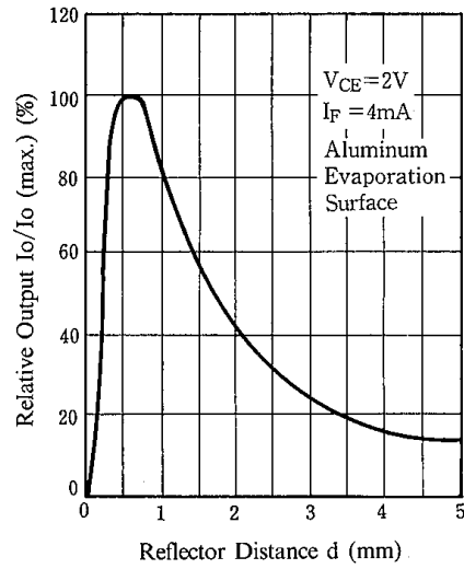
Output Current vs. Distance ( T_a = 25^\circ\text{C} )
