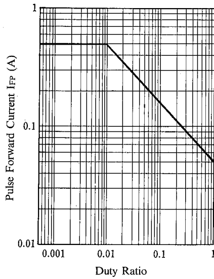
Pulse Forward Current vs. Duty Ratio
