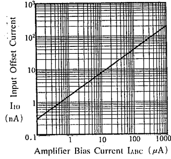
Input Offset Current ( V^+/V^- = \pm 15V , T_a = 25^\circ C )
