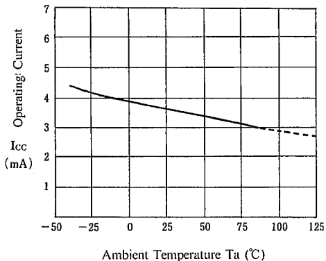
Operating Current vs. Temperature ( V^+/V^- = \pm 15V )
