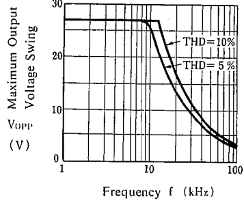
Maximum Output Voltage Swing vs. Frequency ( V^+/V^- = \pm 15V , T_a = 25^\circ C )
