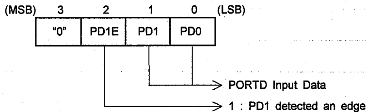
[READING PORTD INPUT DATA (PHY9)]
