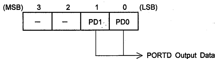
[WRITING PORTD OUTPUT DATA (PHY9)]
