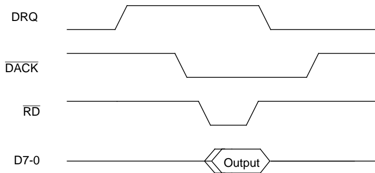
Figure 13. DMA Read from USBN9603
