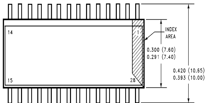
Laminate Substrate Based Package Order Number USBN9603SLB See NS Package Number SLB28AA
