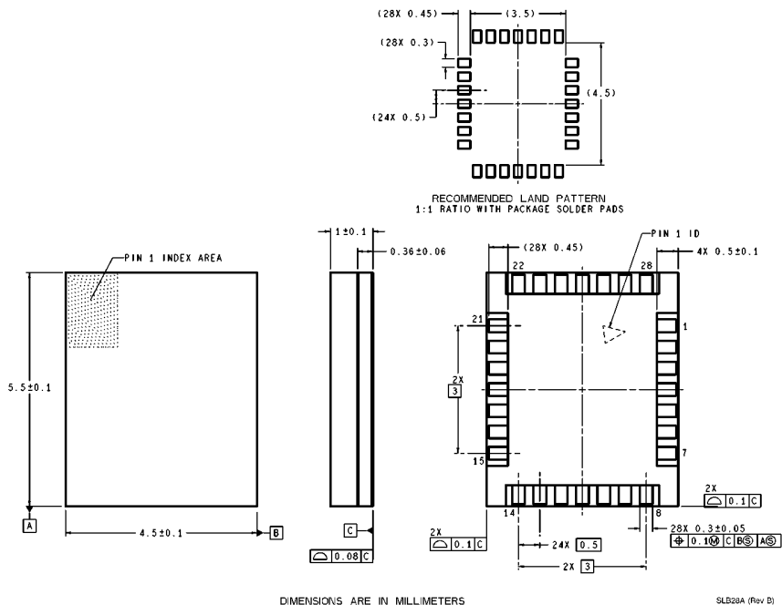
Laminate Substrate Based Package Order Number USBN9603SLB See NS Package Number SLB28AA
