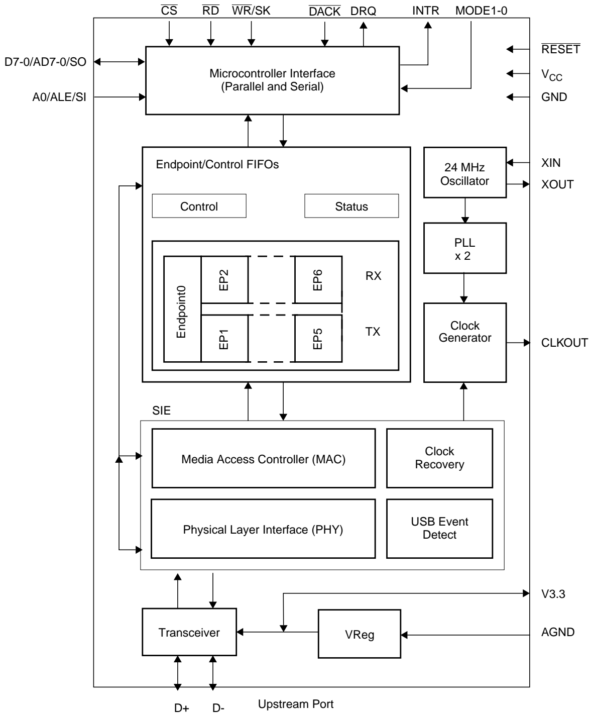
Figure 2. USBN9603 Block Diagram
