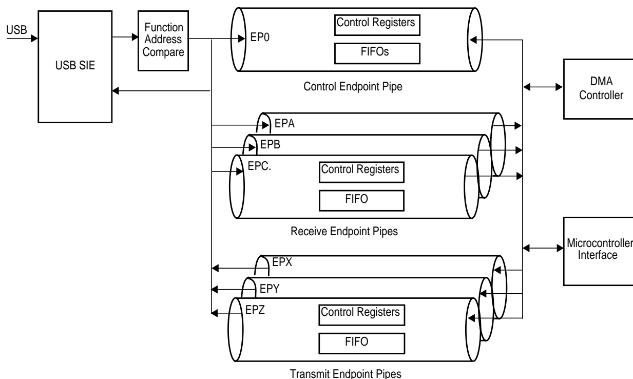
Figure 3. EPC Operation
