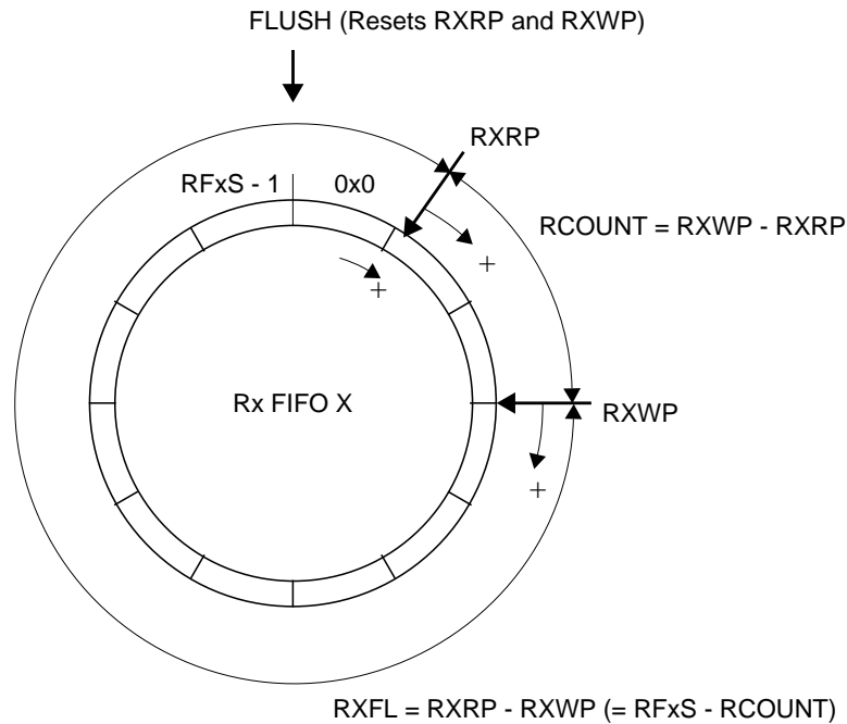
Figure 22. Rx FIFO Operation
