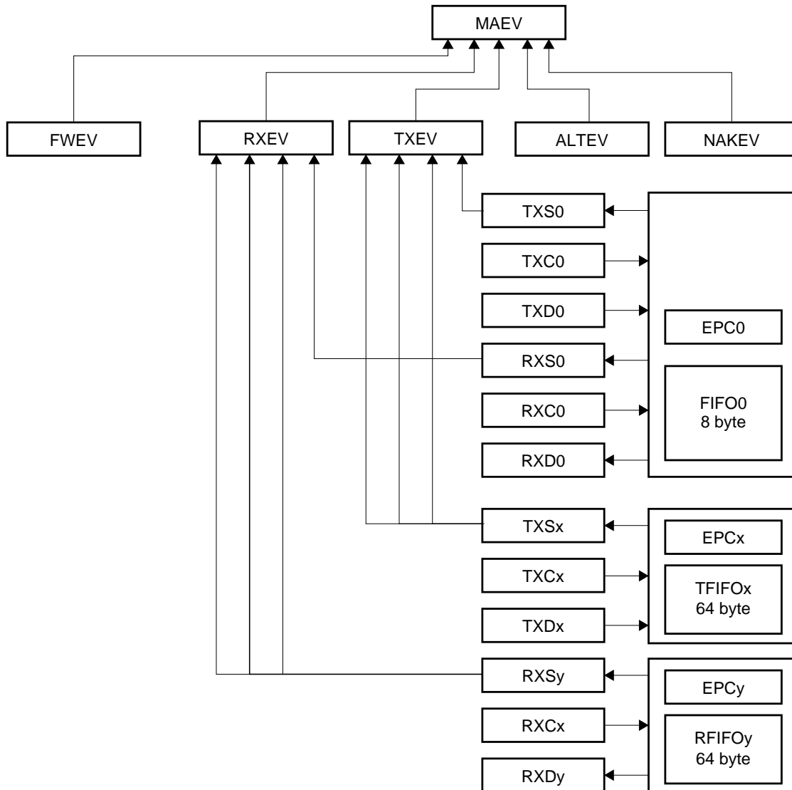
Figure 23. Register Hierarchy
