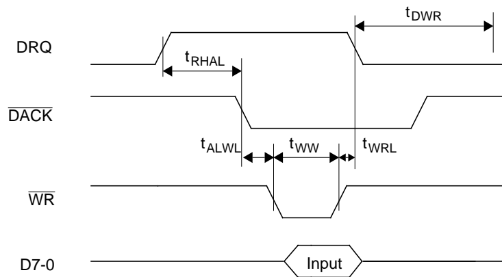
Figure 28. DMA Write to USBN9603
