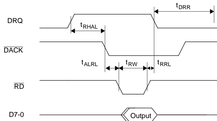
Figure 29. DMA Read to USBN9603
