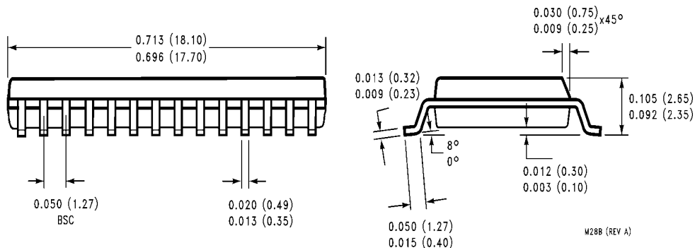
Molded SO Wide Body Package (WM) Order Number USBN9603-28M See NS Package Number M28B
