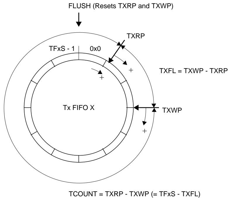
Figure 21. Tx FIFO Operation
