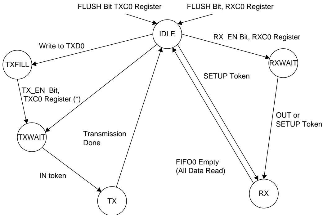
Figure 20. Endpoint 0 Operation
