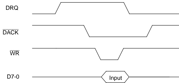
Figure 12. DMA Write to USBN9603
