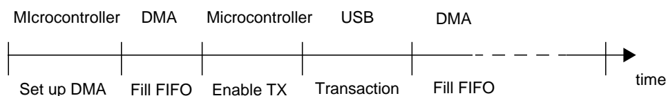
Figure 8. Transmit Operation in Standard DMA Mode
