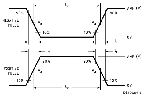
FIGURE 2. V_M = 1.5V
