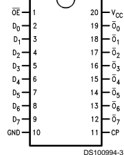
Pin Assignment for DIP, and Flatpak
