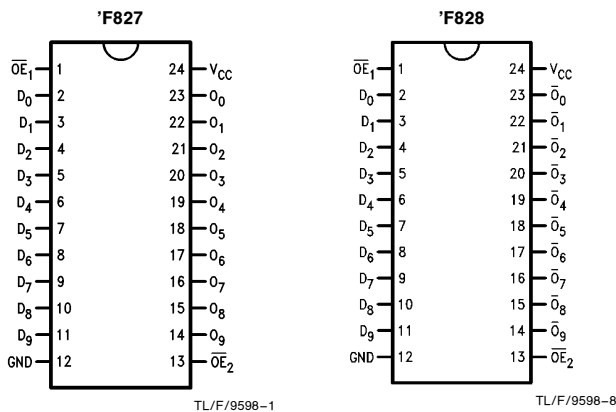
Pin Assignment for DIP, Flatpak and SOIC
