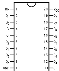
Pin Assignment for DIP and Flatpack
