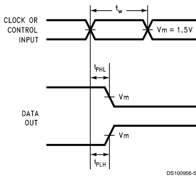
FIGURE 2. Propagation Delay, Pulse Width Waveforms
