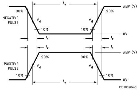
FIGURE 2. V_M = 1.5V
