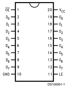
Pin Assignment for DIP and Cerpack
