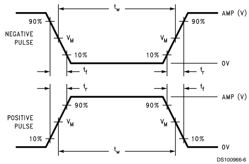
FIGURE 2. V_M = 1.5V
